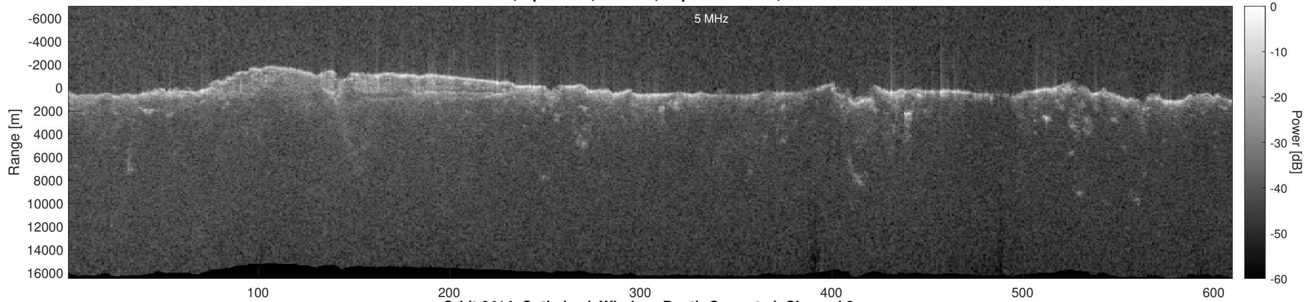
Orbit 6414, Optimized, Window, Depth-Corrected, Channel 2
