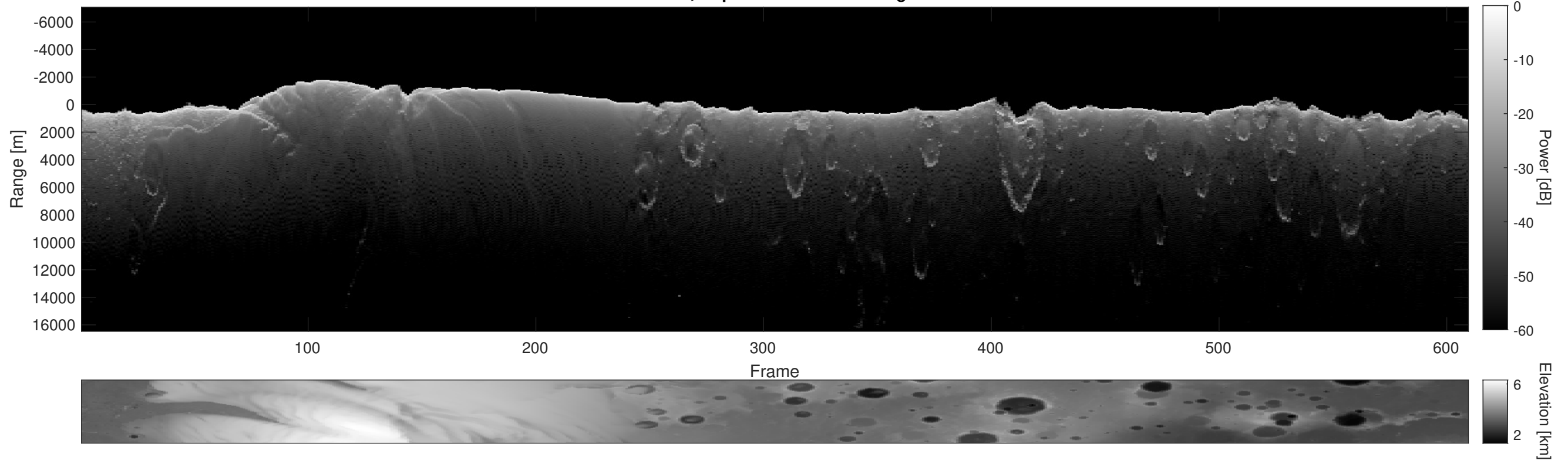
Orbit 6414, Depth-Corrected Cluttergram
