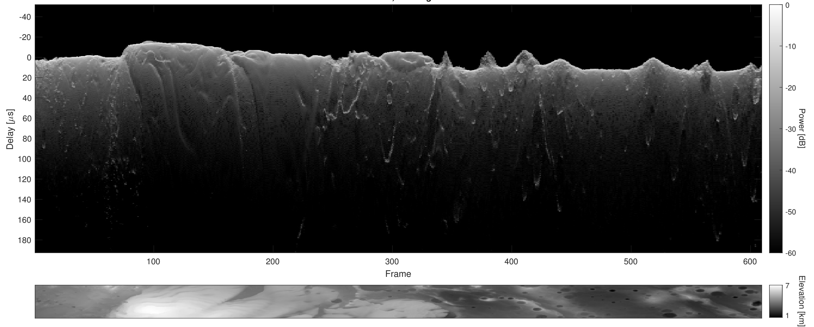
Orbit 6415, Cluttergram
