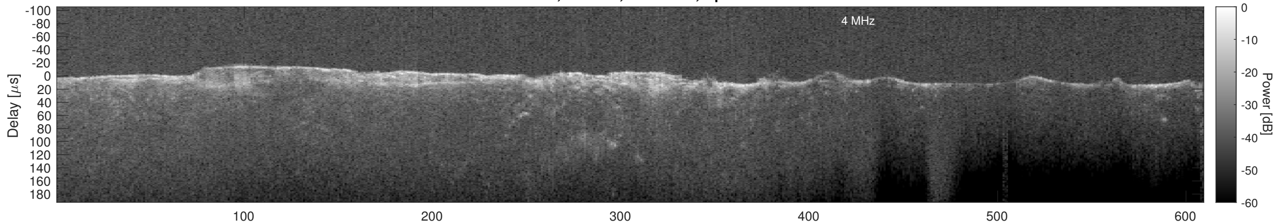
Orbit 6415, Cluttergram
