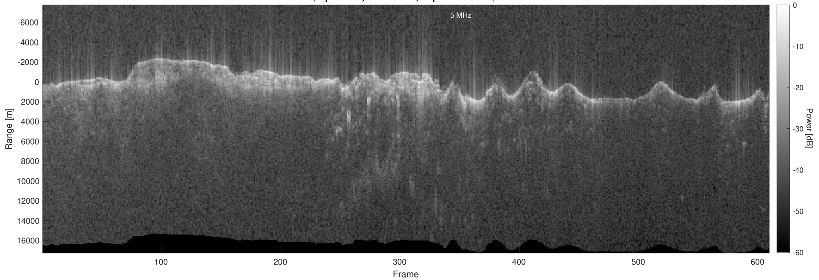
Orbit 6415, Optimized, No Window, Depth-Corrected, Channel 2
