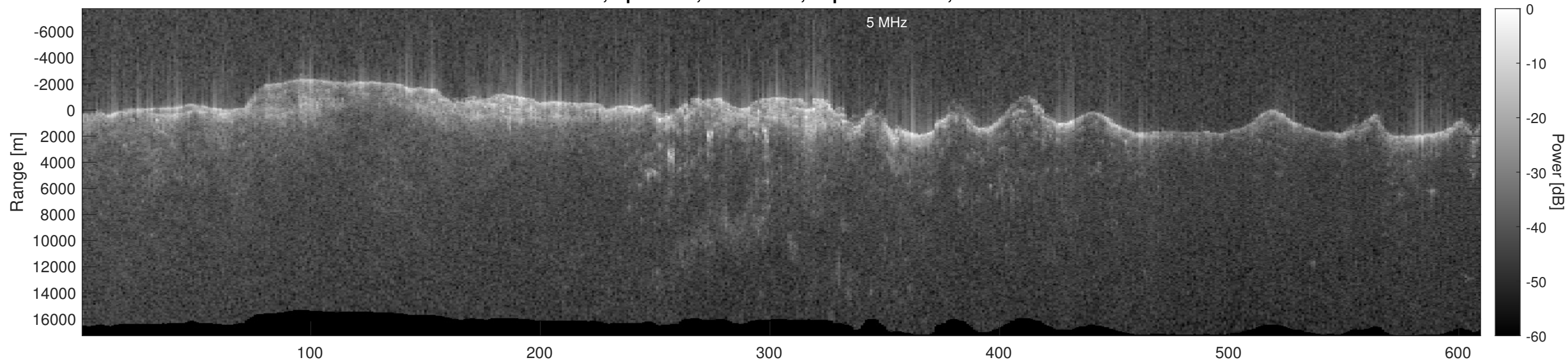
Orbit 6415, Optimized, No Window, Depth-Corrected, Channel 2
