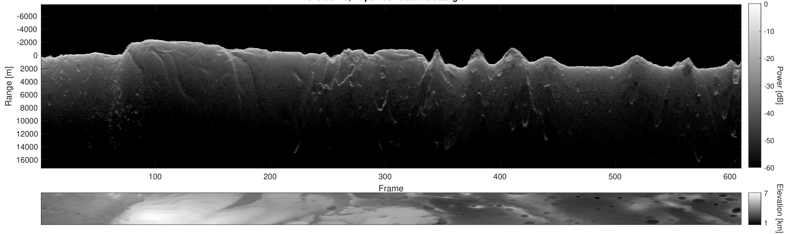
Orbit 6415, Depth-Corrected Cluttergram
