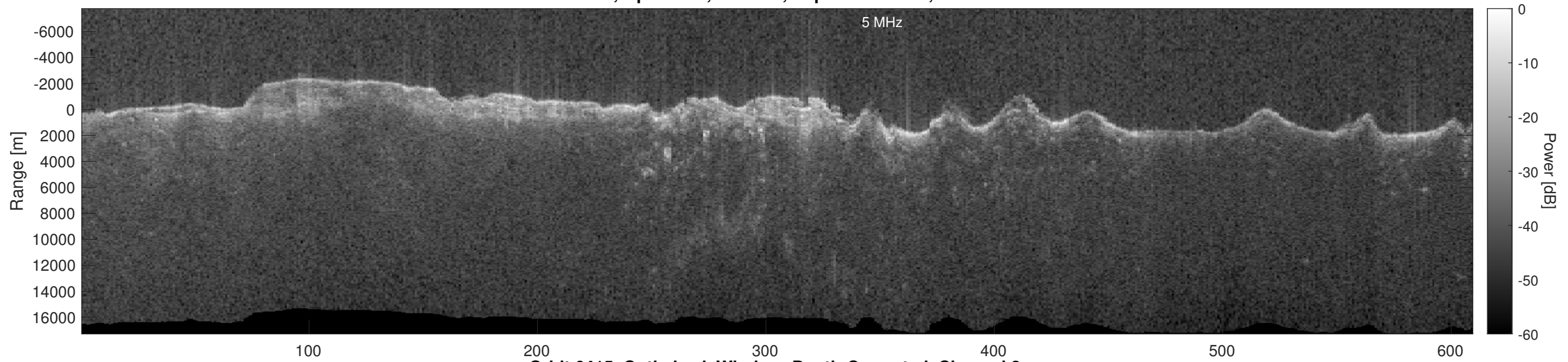
Orbit 6415, Optimized, Window, Depth-Corrected, Channel 2
