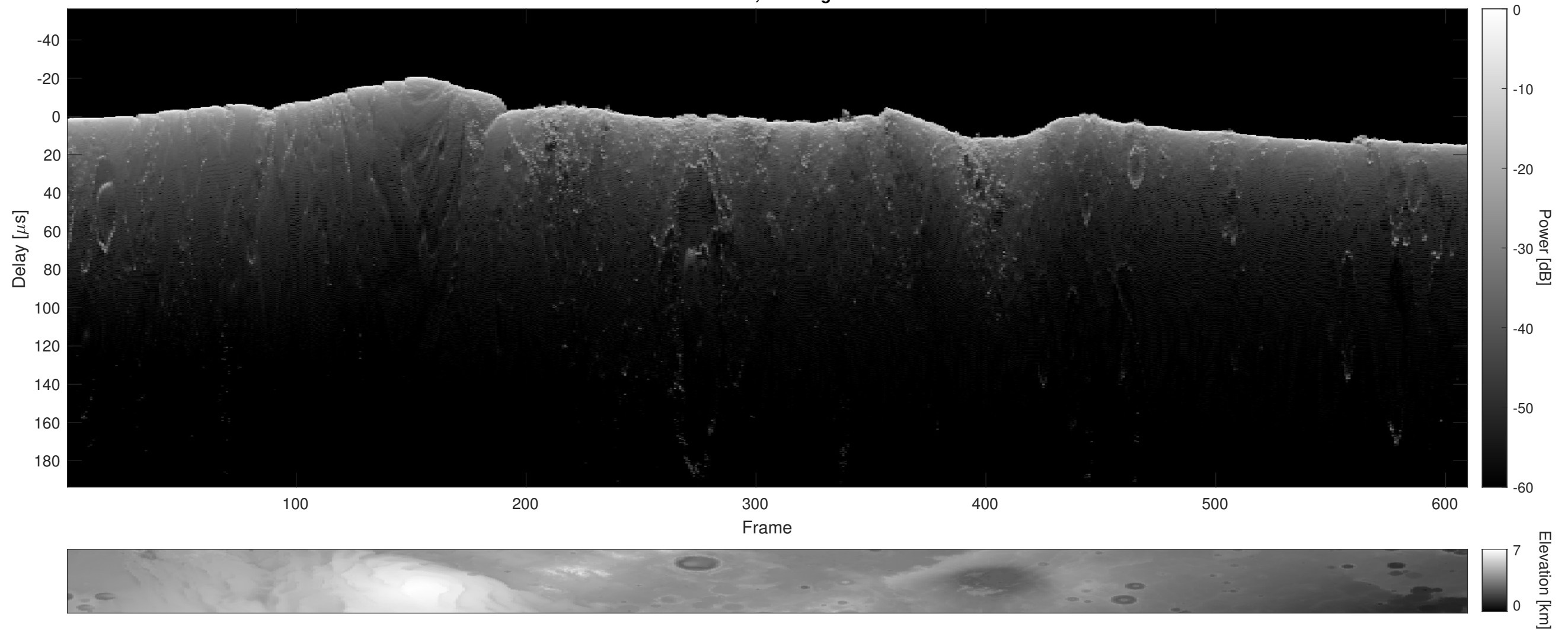
Orbit 6416, Cluttergram
