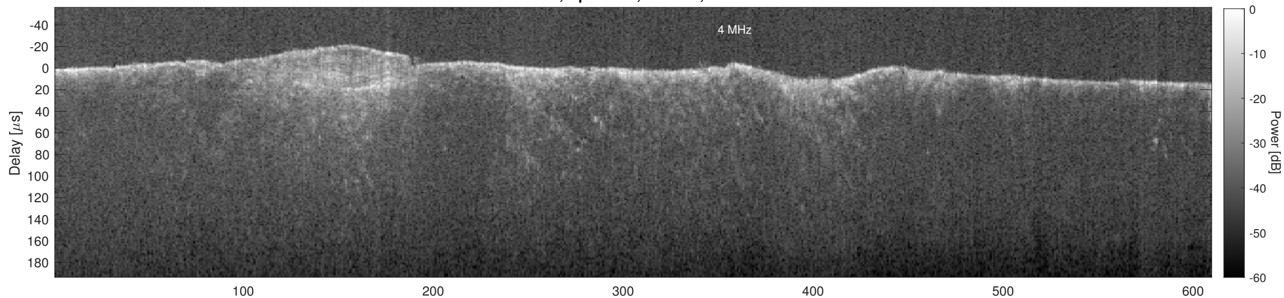
Orbit 6416, Cluttergram
