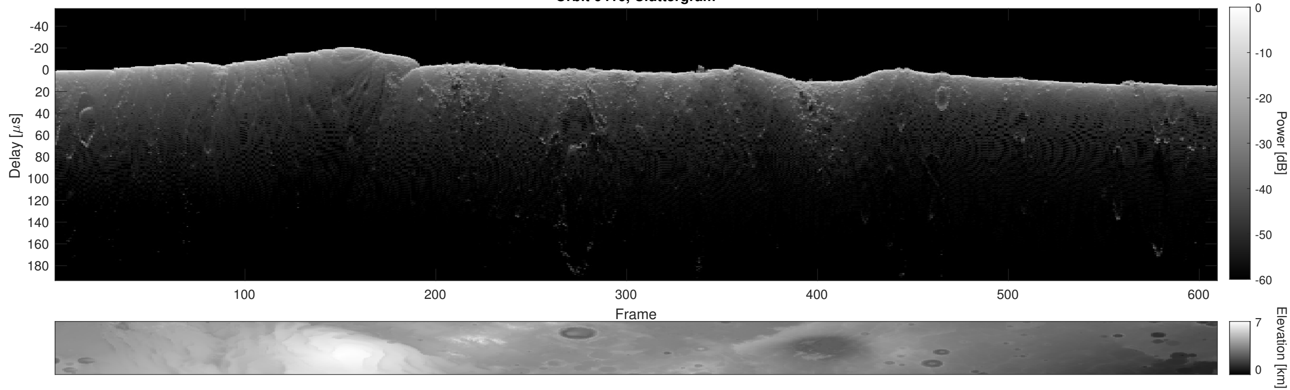
Orbit 6416, Cluttergram
