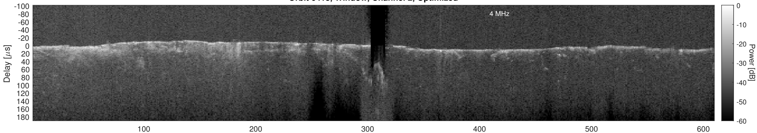
Orbit 6418, Cluttergram
