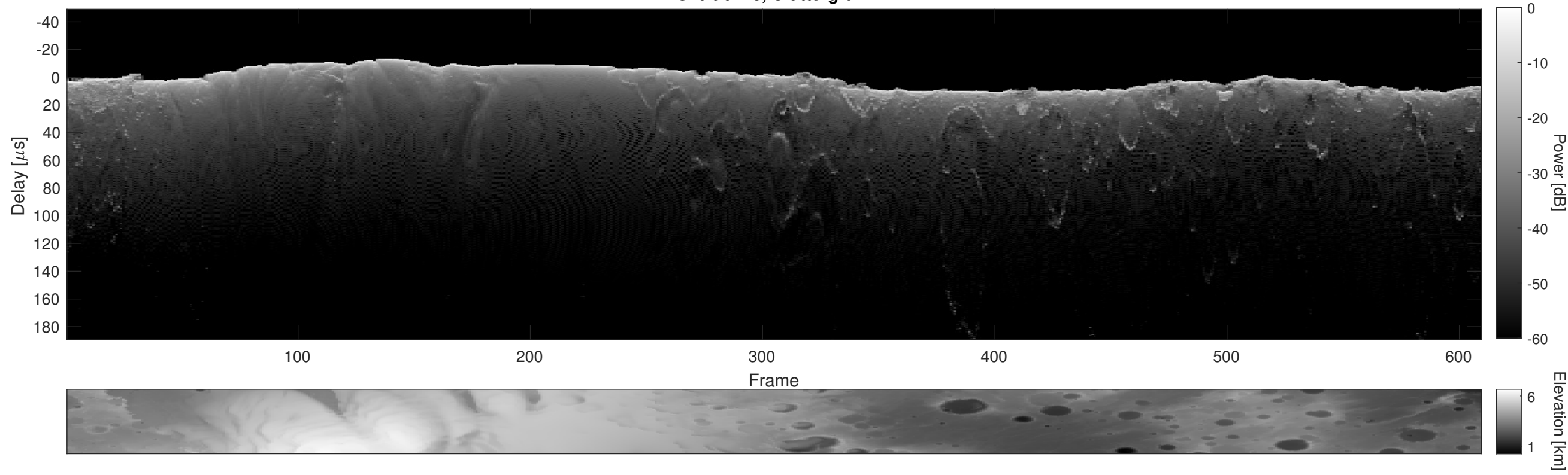
Orbit 6418, Cluttergram
