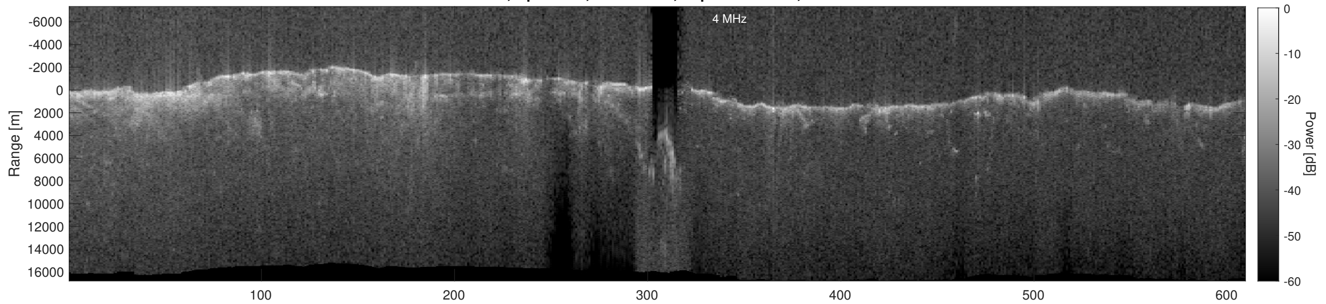
Orbit 6418, Depth-Corrected Cluttergram
