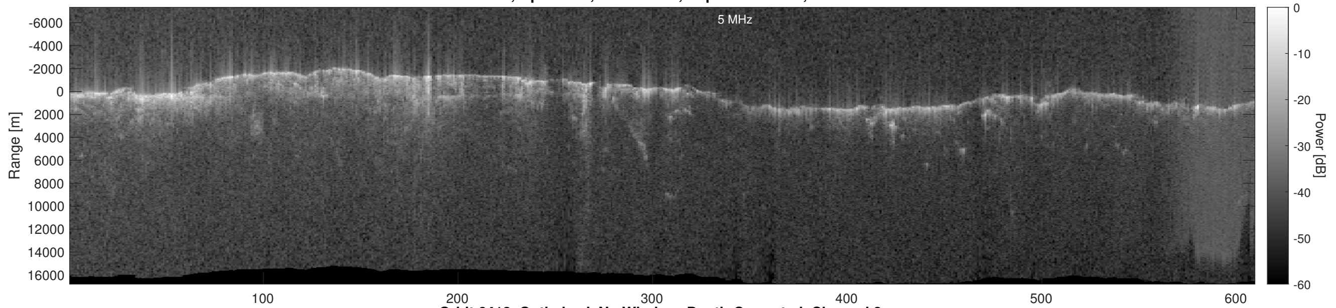
Orbit 6418, Optimized, No Window, Depth-Corrected, Channel 2
