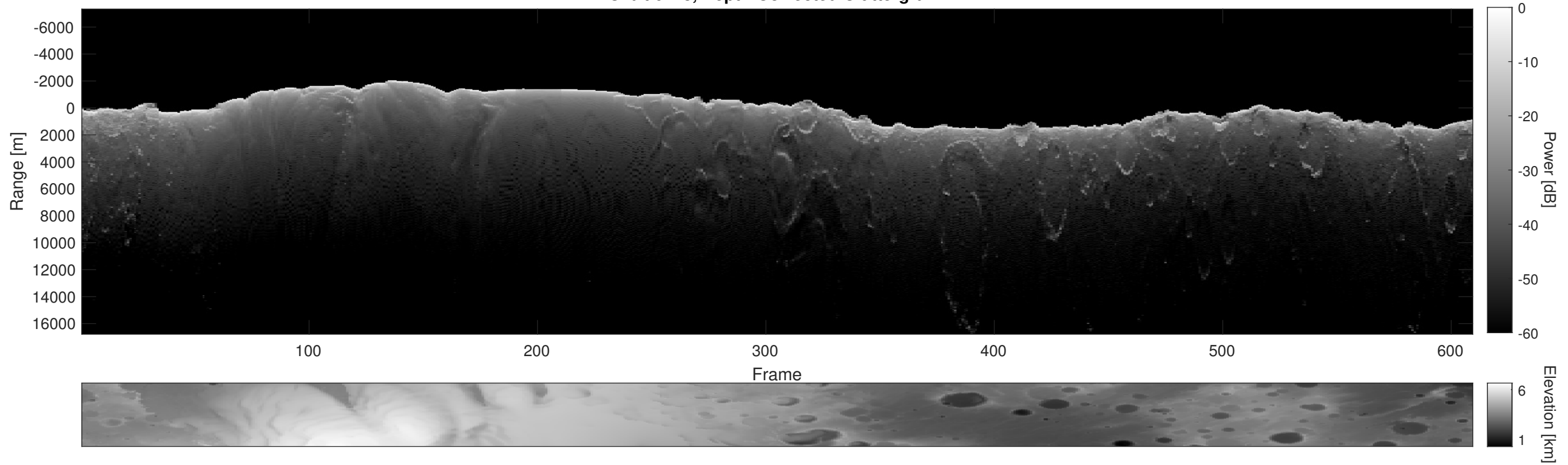
Orbit 6418, Depth-Corrected Cluttergram
