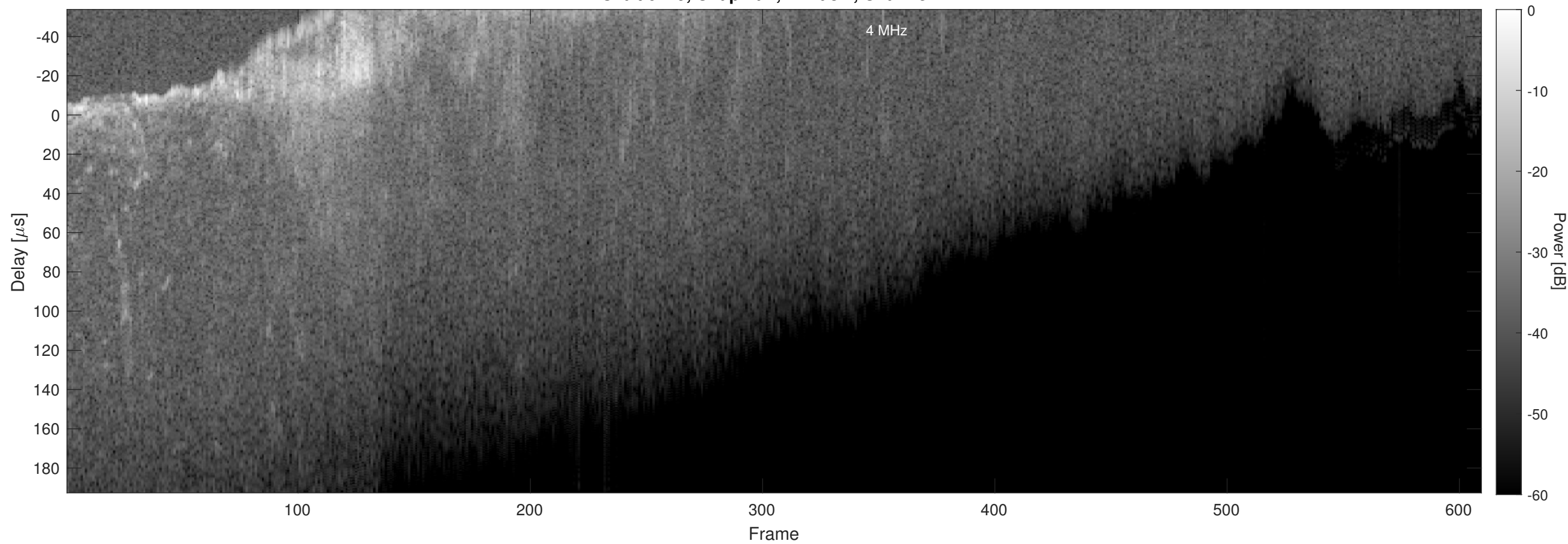
Orbit 6419, Chapman, Window, Channel 2
