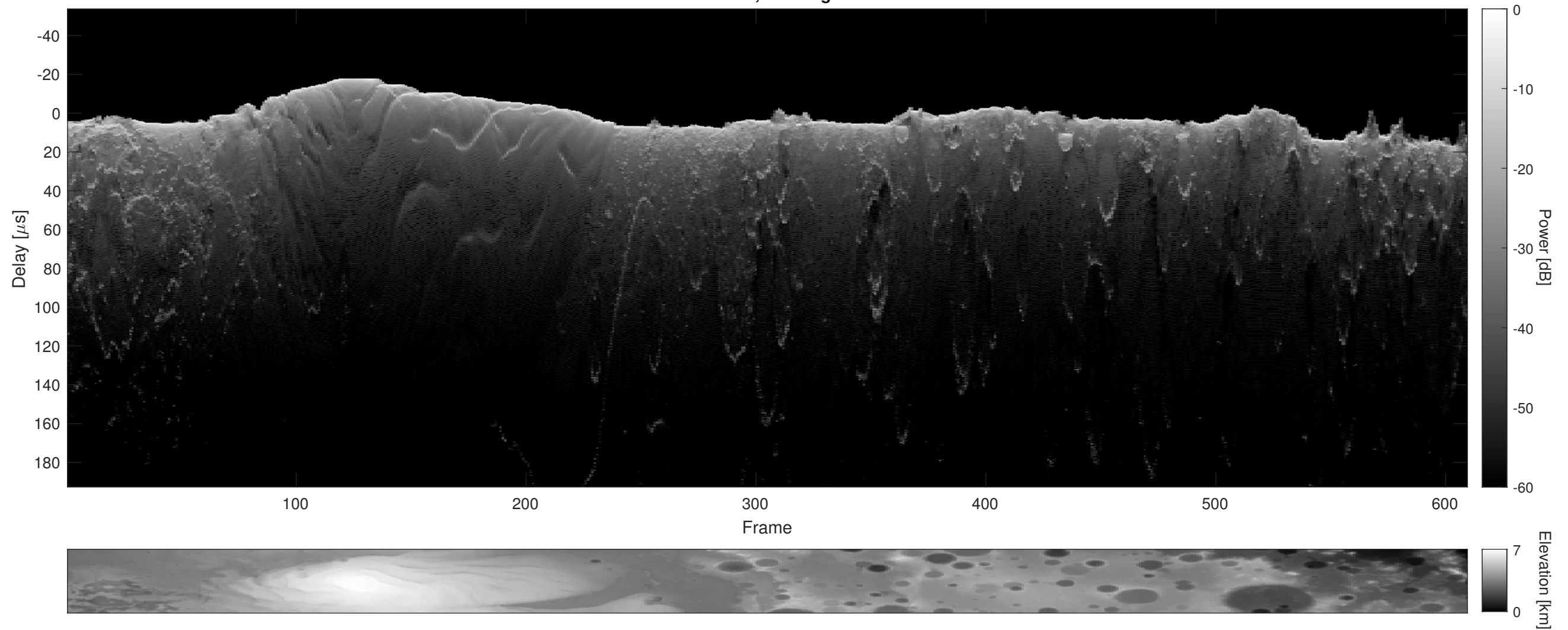
Orbit 6419, Cluttergram
