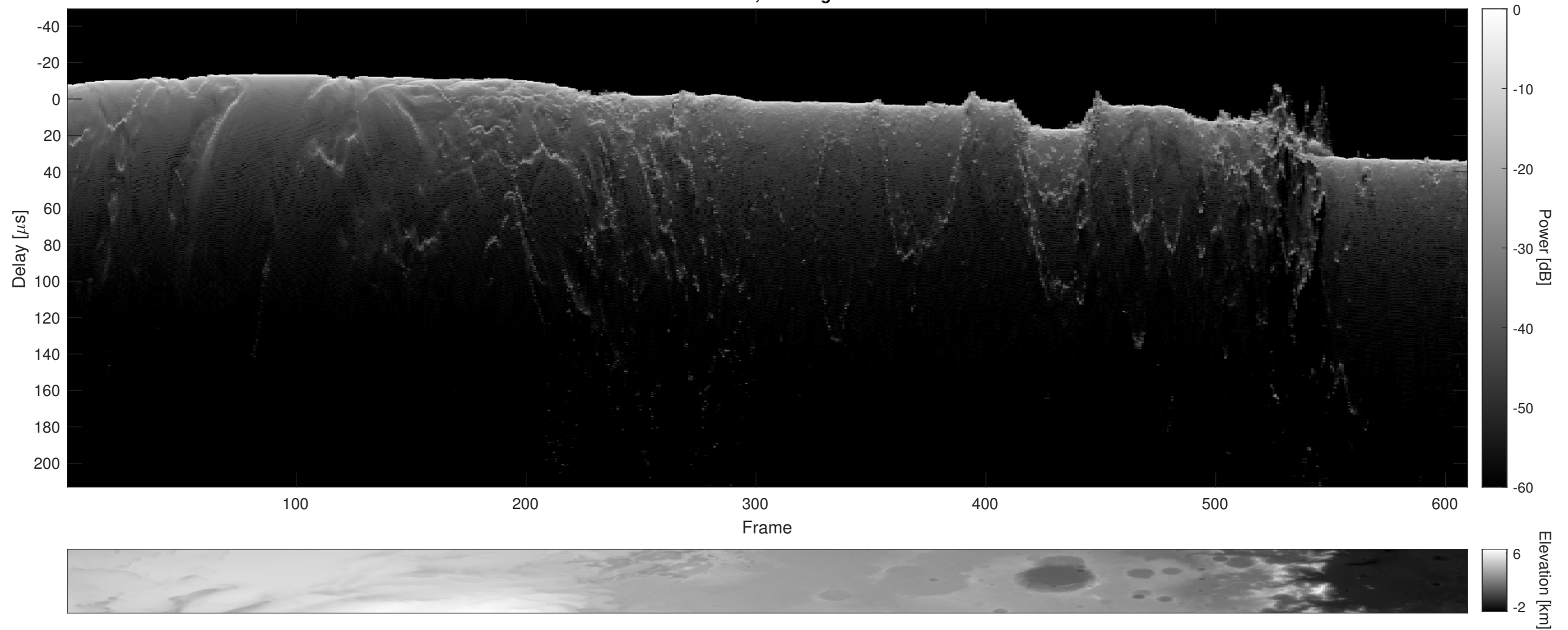
Orbit 6424, Cluttergram
