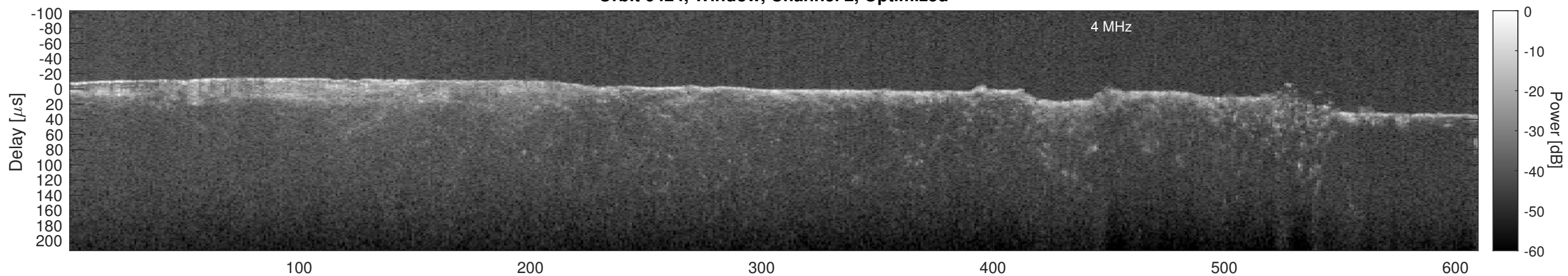
Orbit 6424, Cluttergram
