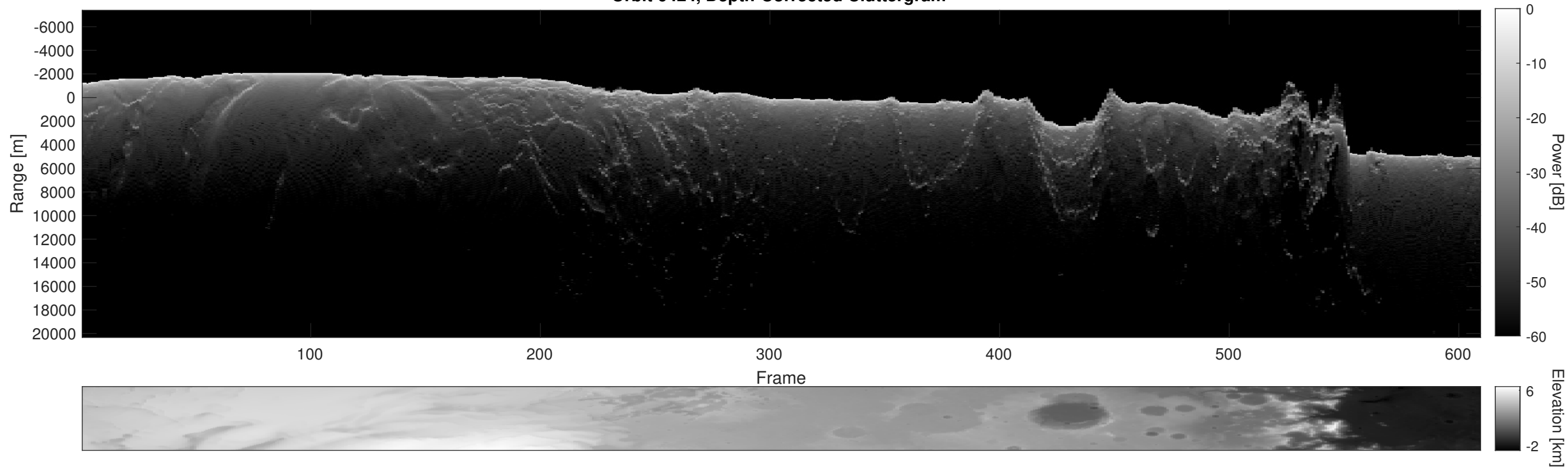
Orbit 6424, Depth-Corrected Cluttergram
