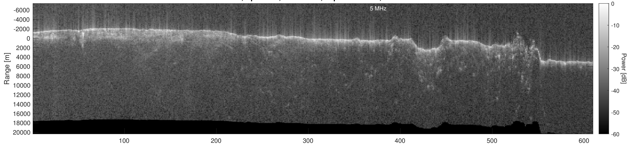
Orbit 6424, Optimized, No Window, Depth-Corrected, Channel 2
