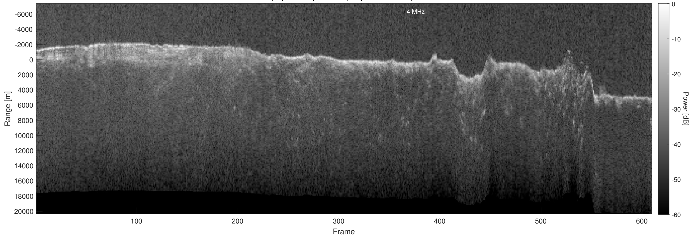
Orbit 6424, Optimized, Window, Depth-Corrected, Channel 2
