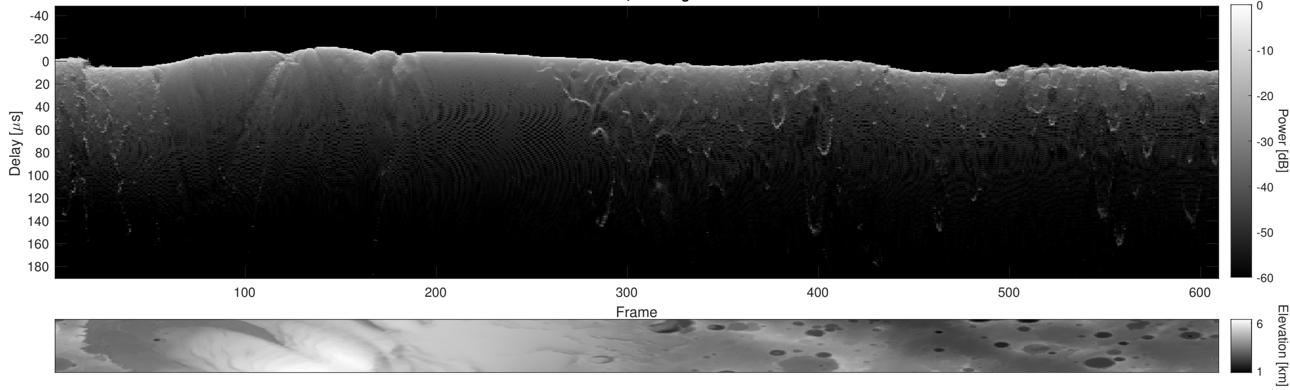
Orbit 6425, Cluttergram
