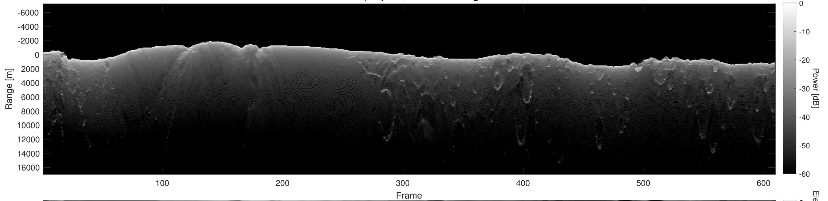
Orbit 6425, Depth-Corrected Cluttergram
