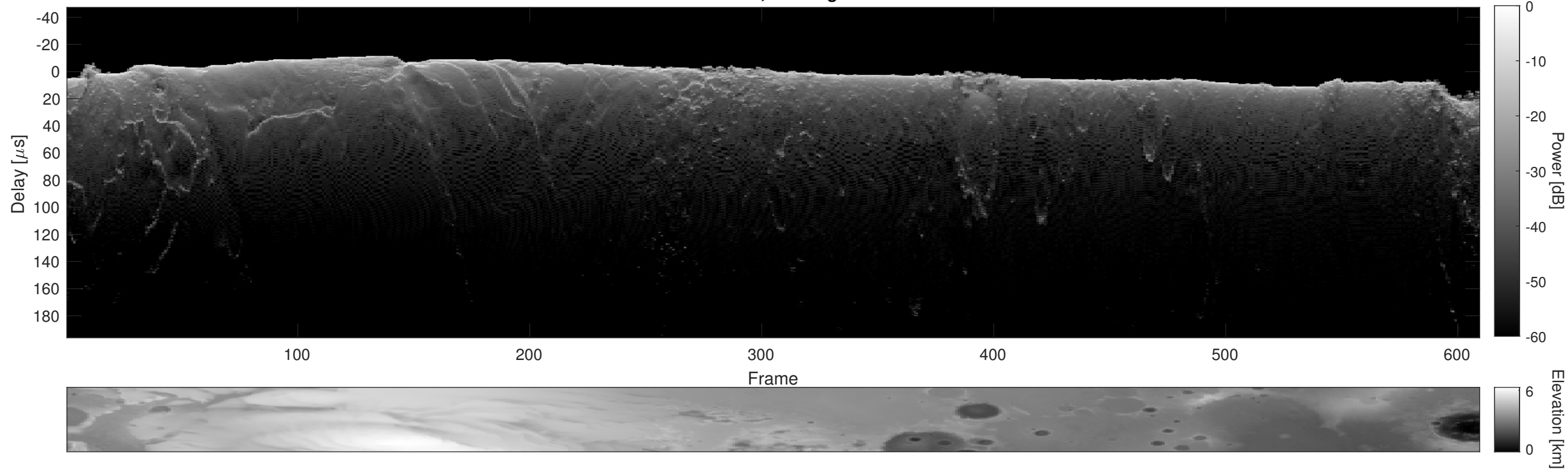
Orbit 6428, Cluttergram
