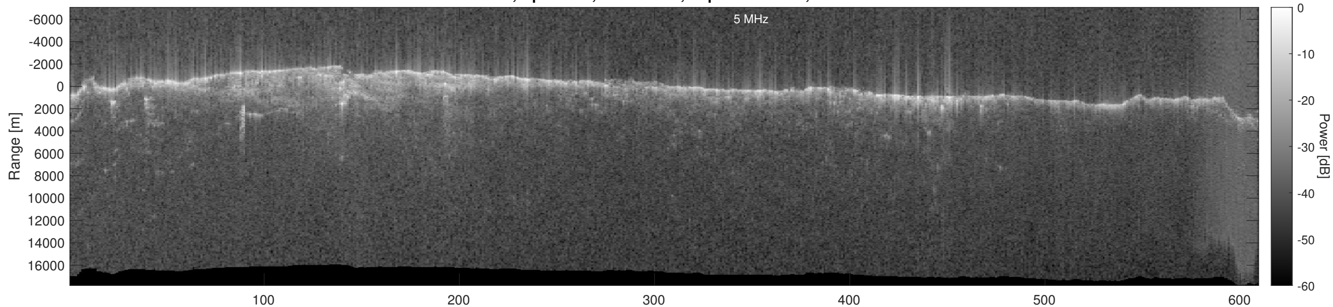
Orbit 6428, Optimized, No Window, Depth-Corrected, Channel 2
