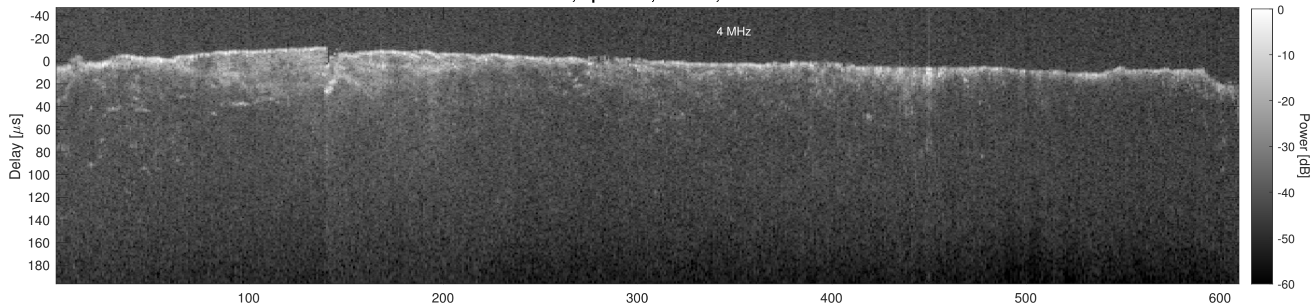
Orbit 6428, Cluttergram
