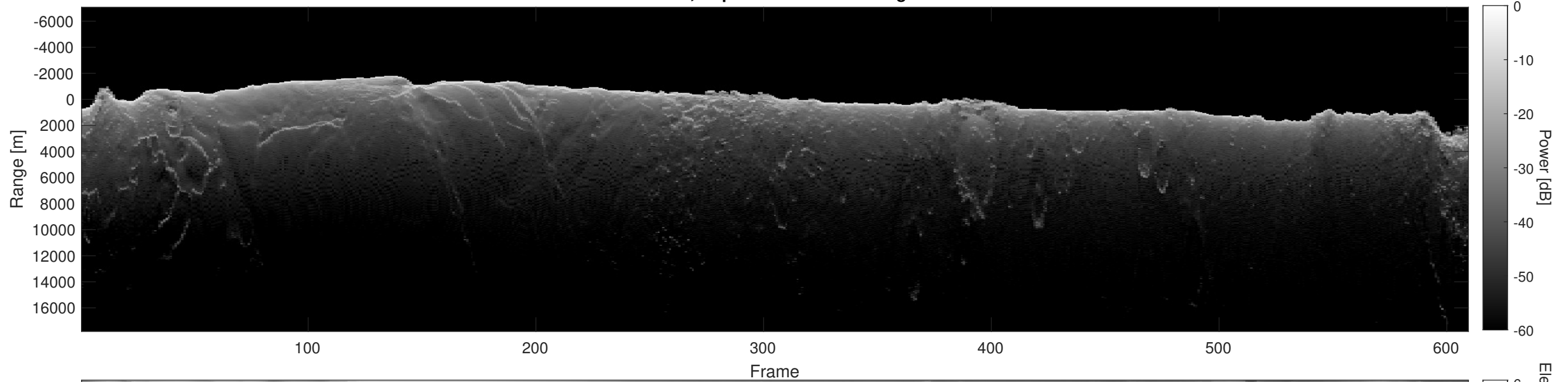
Orbit 6428, Depth-Corrected Cluttergram
