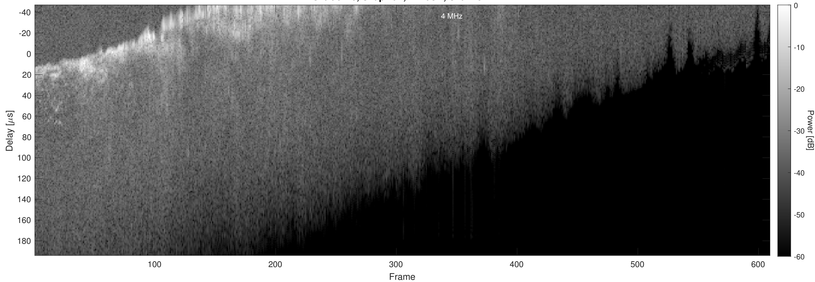
Orbit 6429, Chapman, Window, Channel 2
