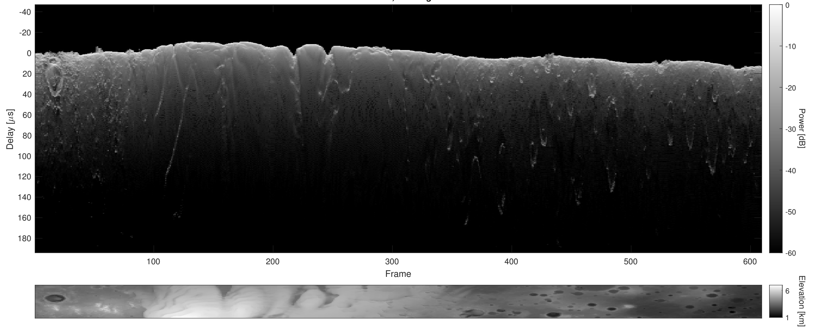
Orbit 6429, Cluttergram
