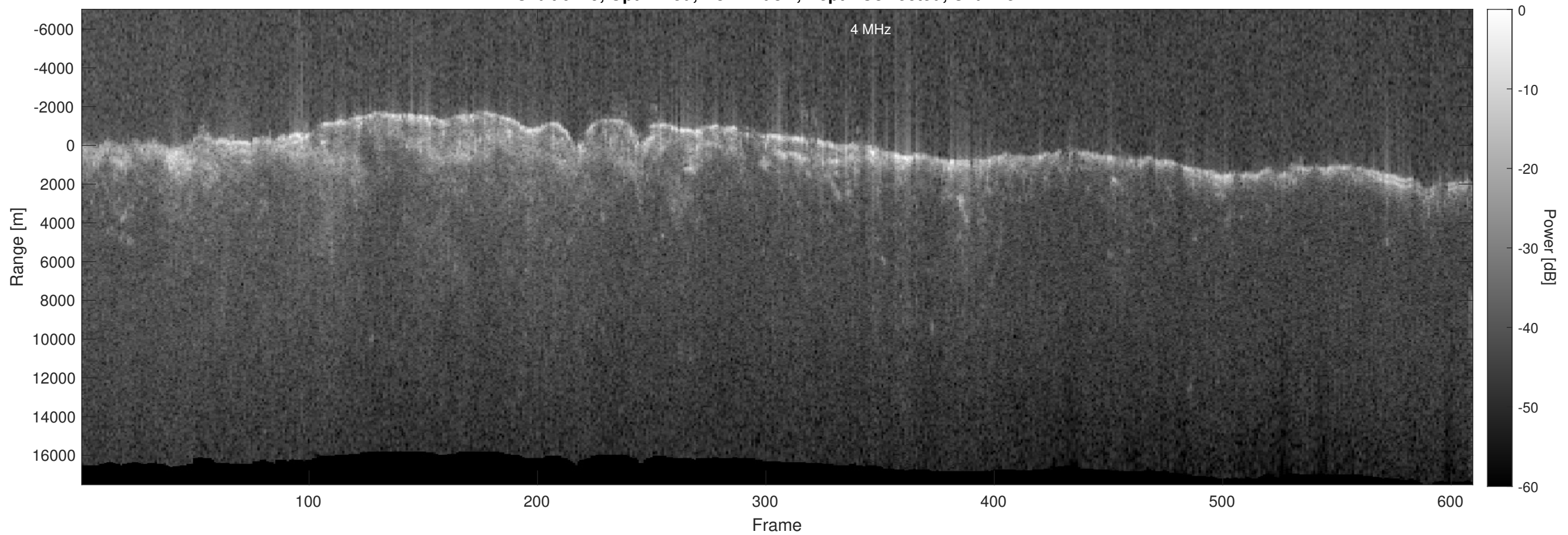
Orbit 6429, Optimized, No Window, Depth-Corrected, Channel 2
