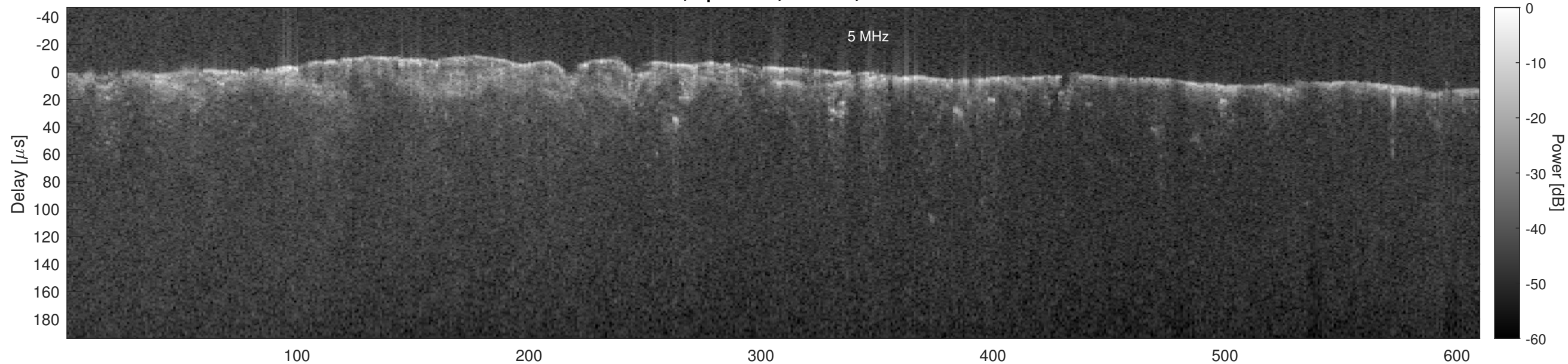
Orbit 6429, Optimized, Window, Channel 2
