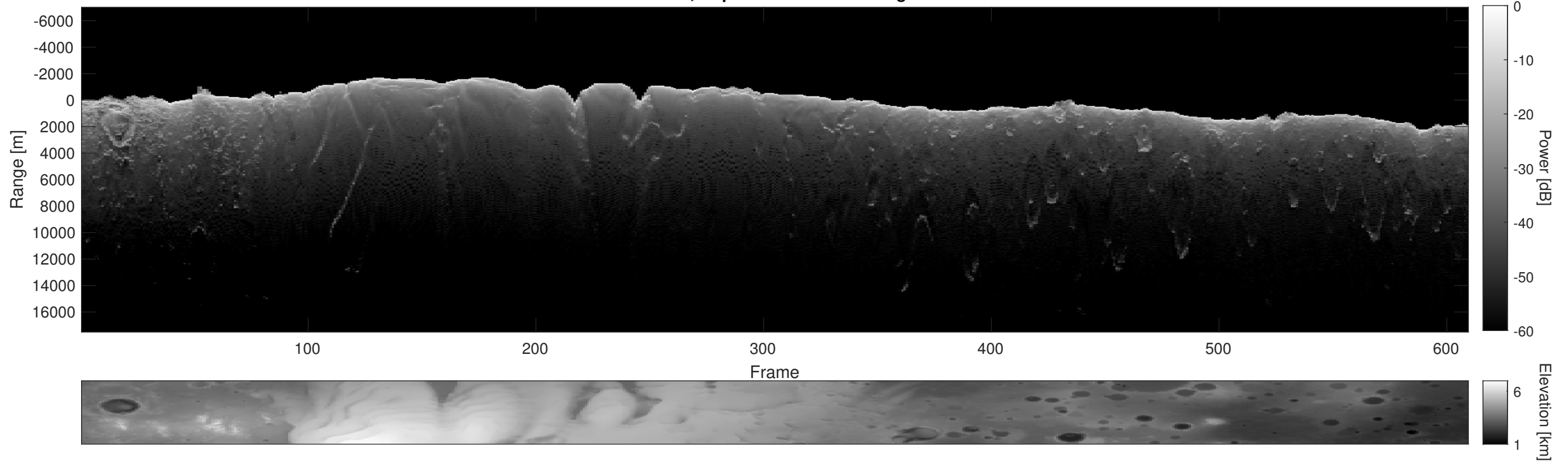
Orbit 6429, Depth-Corrected Cluttergram
