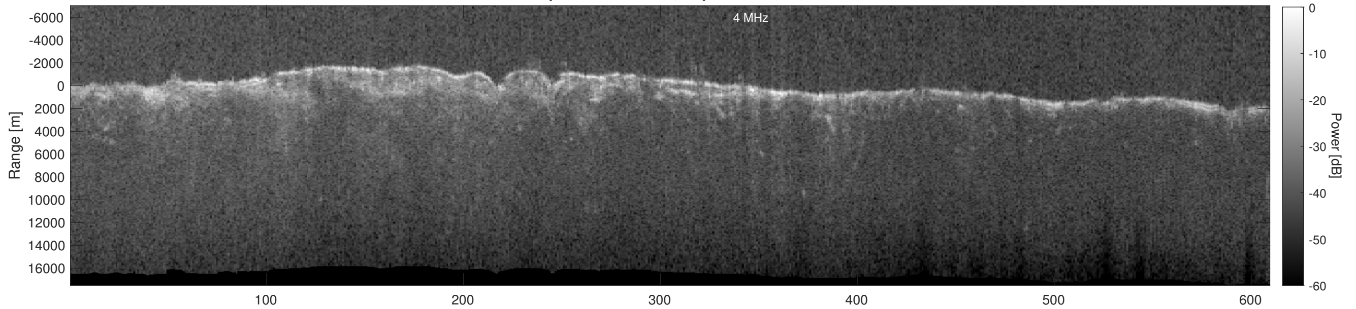
Orbit 6429, Depth-Corrected Cluttergram
