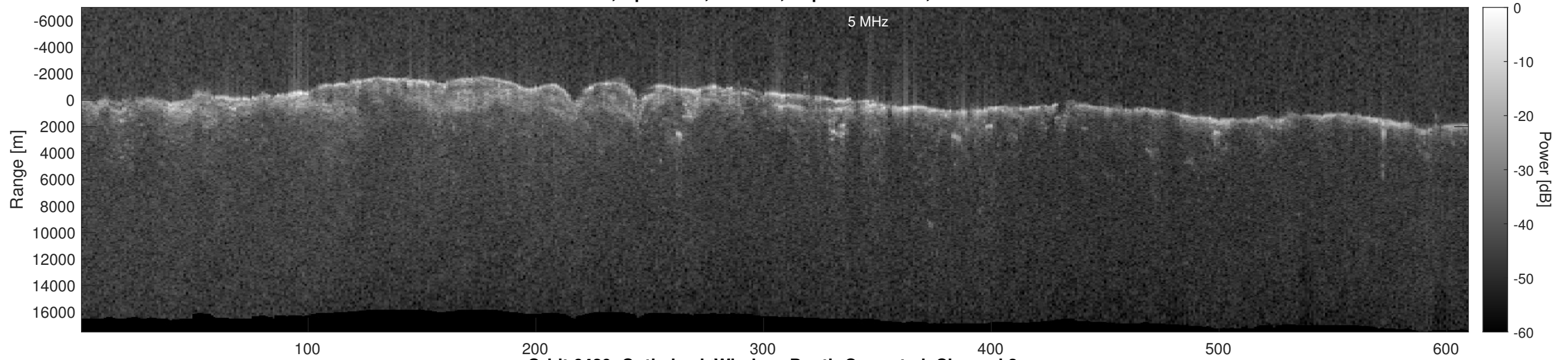
Orbit 6429, Optimized, Window, Depth-Corrected, Channel 2
