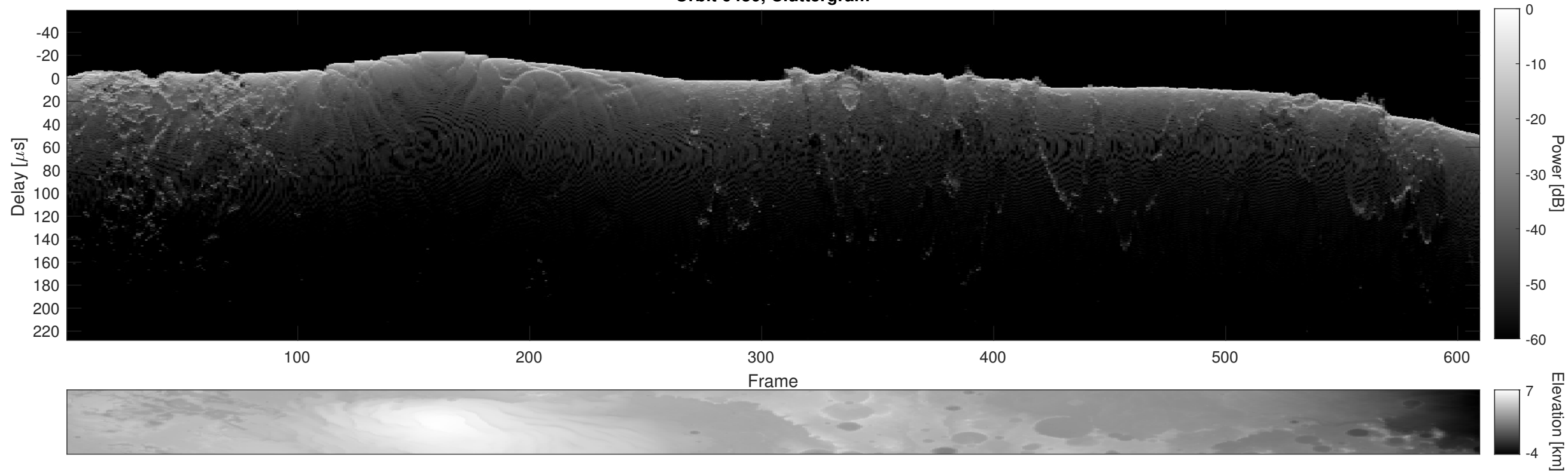
Orbit 6430, Cluttergram
