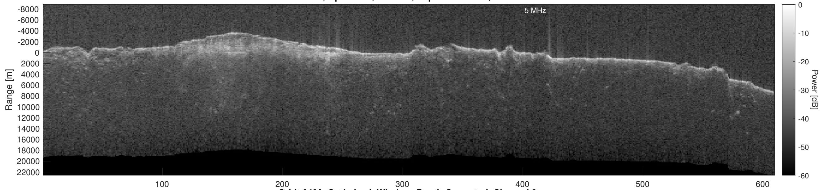
Orbit 6430, Optimized, Window, Depth-Corrected, Channel 2
