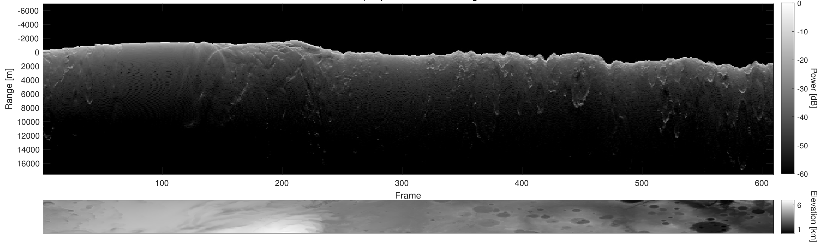
Orbit 6431, Depth-Corrected Cluttergram
