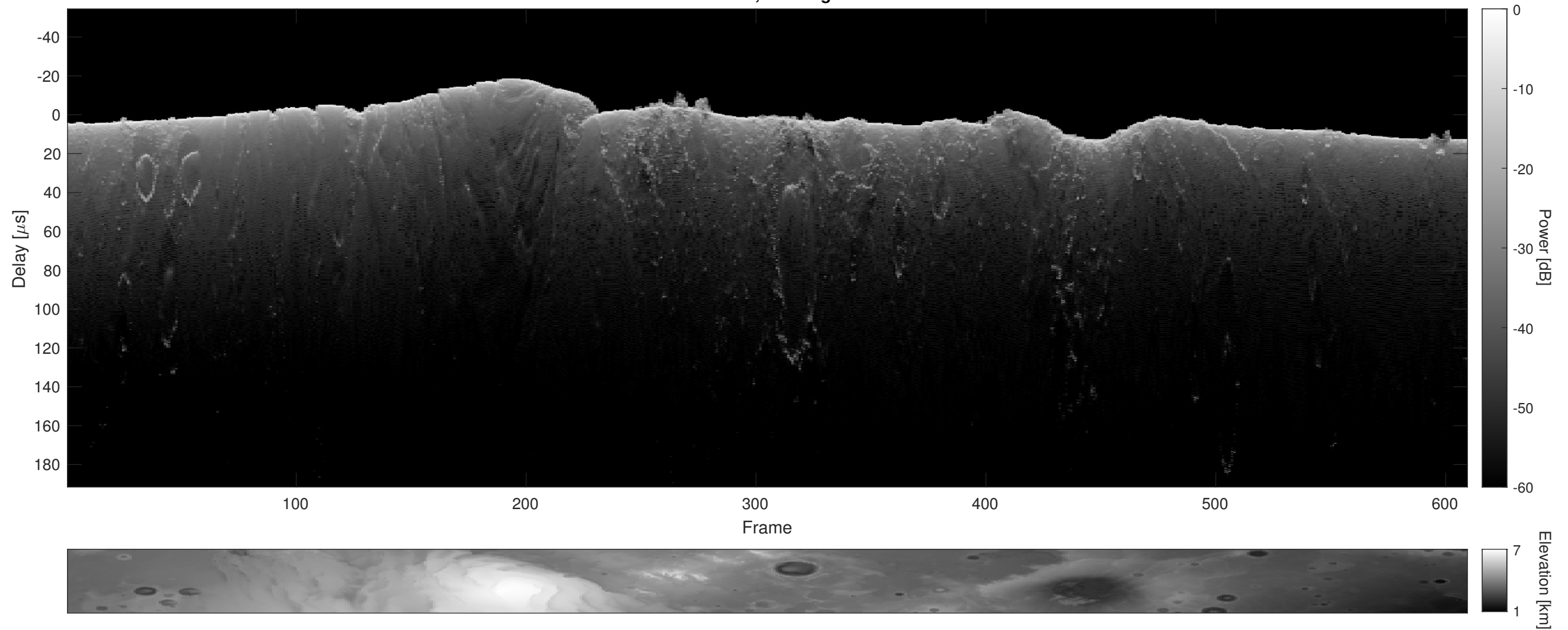
Orbit 6434, Cluttergram
