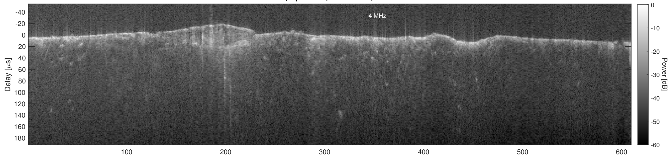
Orbit 6434, Cluttergram
