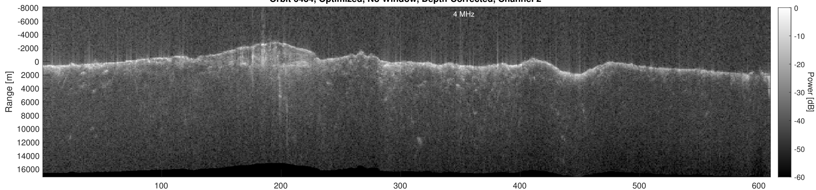
Orbit 6434, Depth-Corrected Cluttergram
