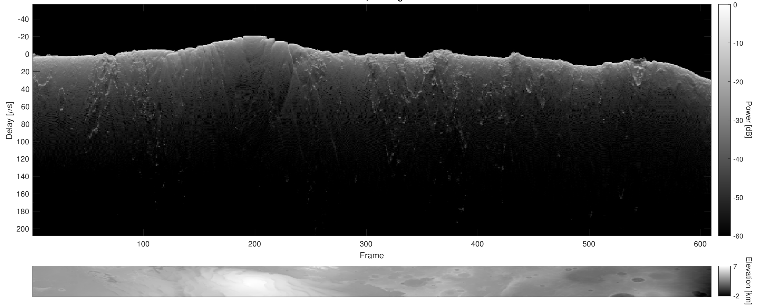
Orbit 6441, Cluttergram
