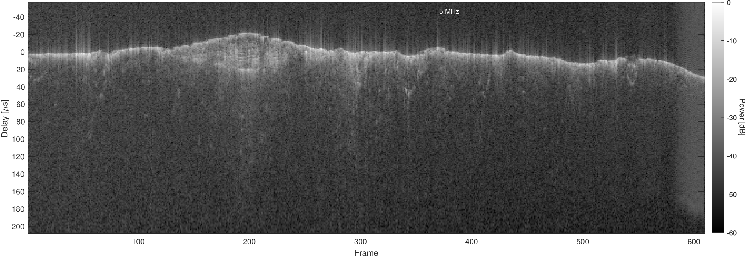
Orbit 6441, Optimized, No Window, Channel 2
