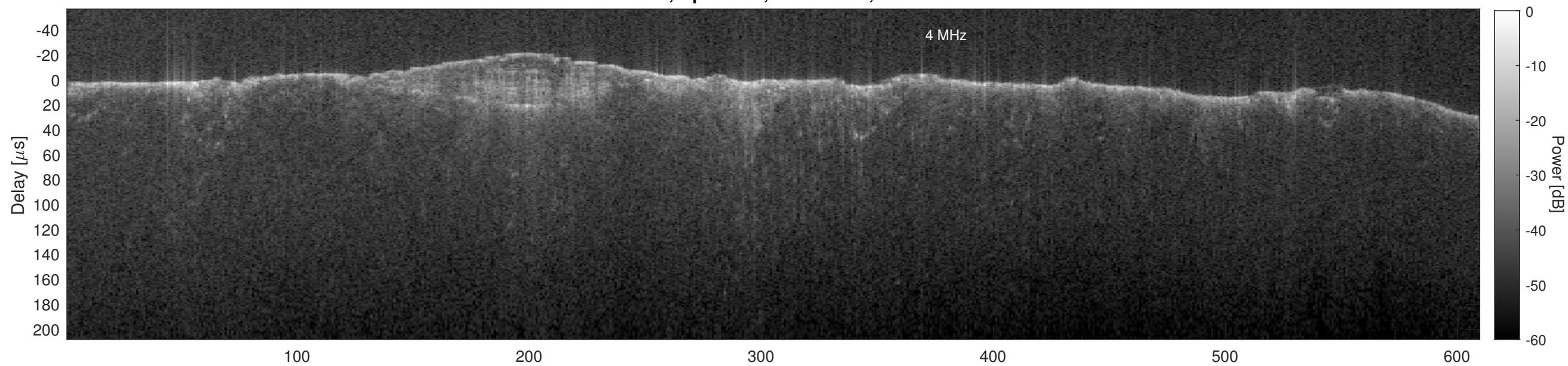
Orbit 6441, Cluttergram
