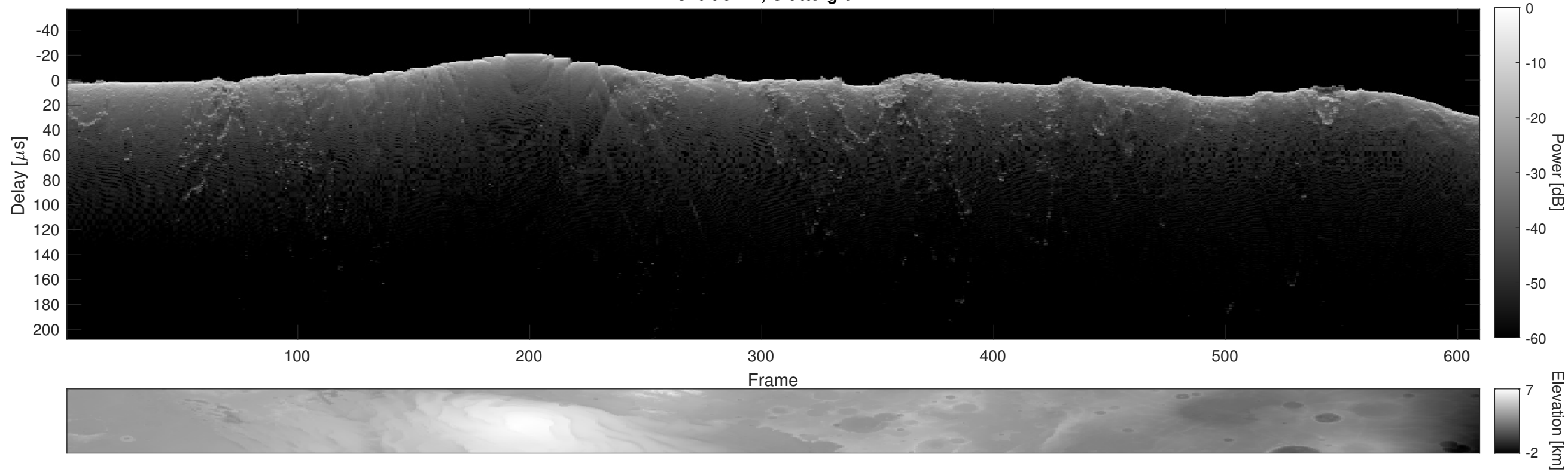
Orbit 6441, Cluttergram
