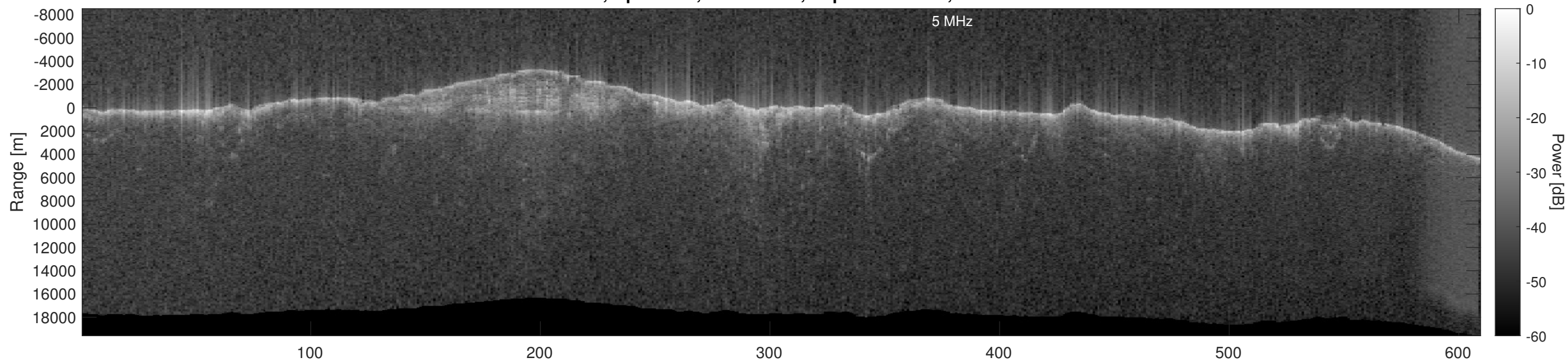
Orbit 6441, Optimized, No Window, Depth-Corrected, Channel 2
