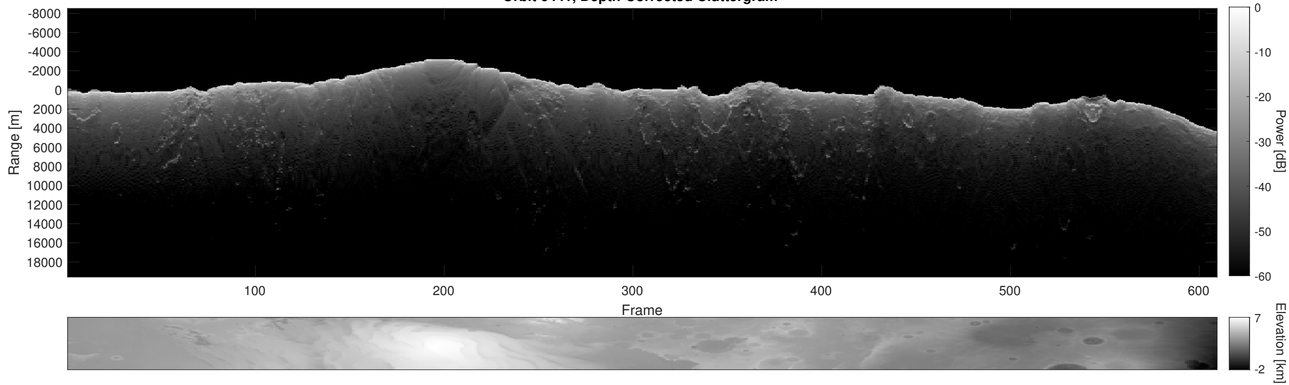
Orbit 6441, Depth-Corrected Cluttergram
