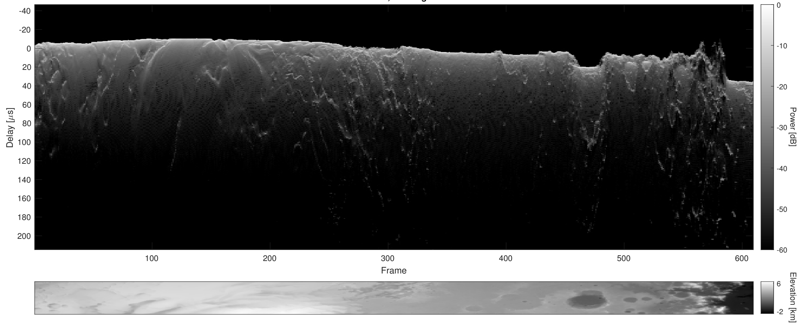
Orbit 6442, Cluttergram
