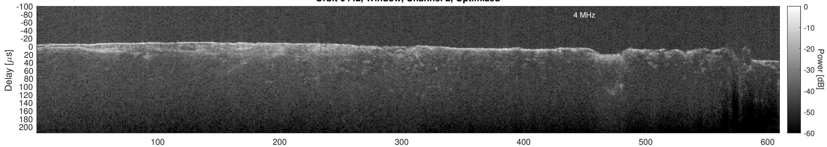
Orbit 6442, Cluttergram
