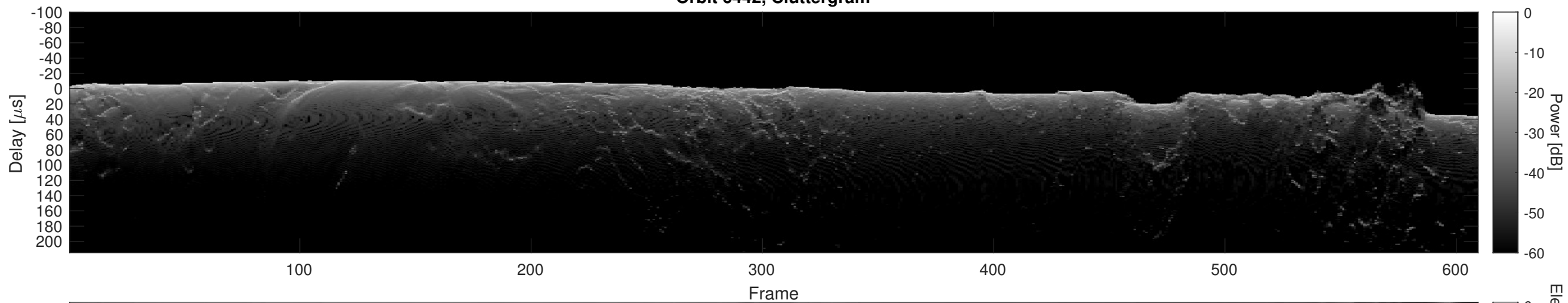
Orbit 6442, Cluttergram
