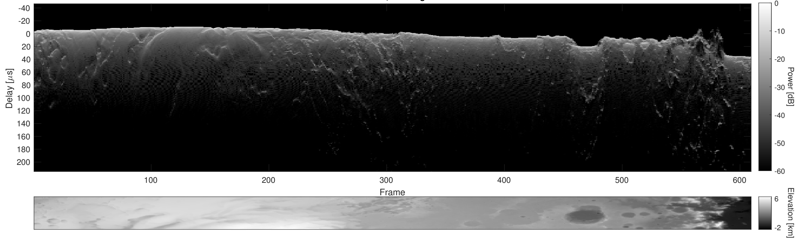
Orbit 6442, Cluttergram
