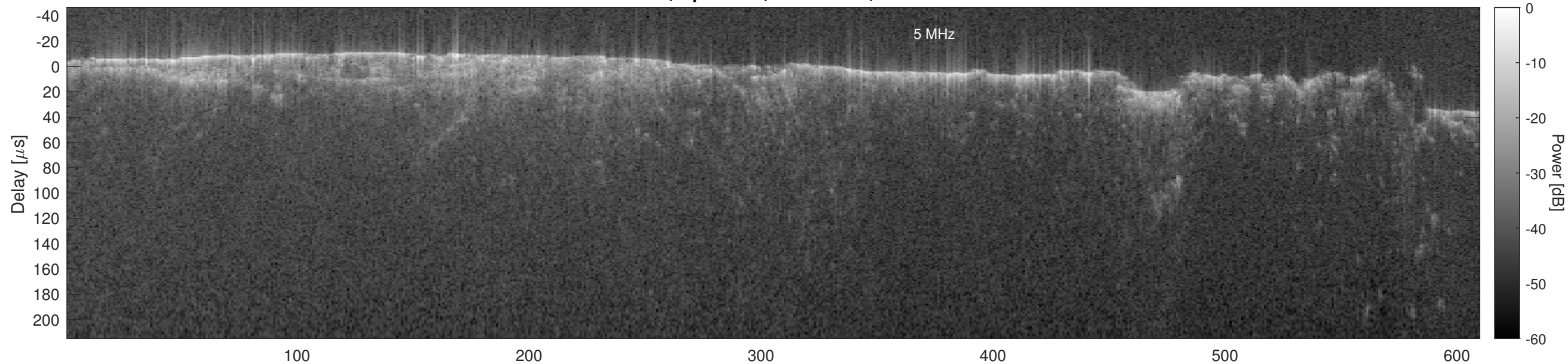
Orbit 6442, Optimized, No Window, Channel 2
