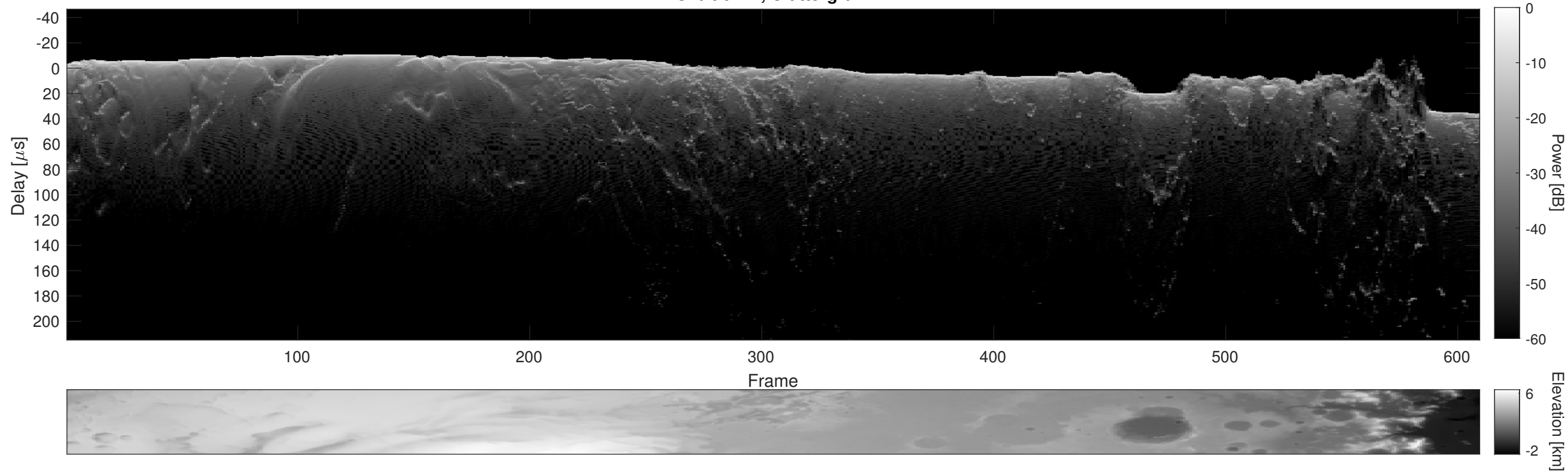
Orbit 6442, Cluttergram
