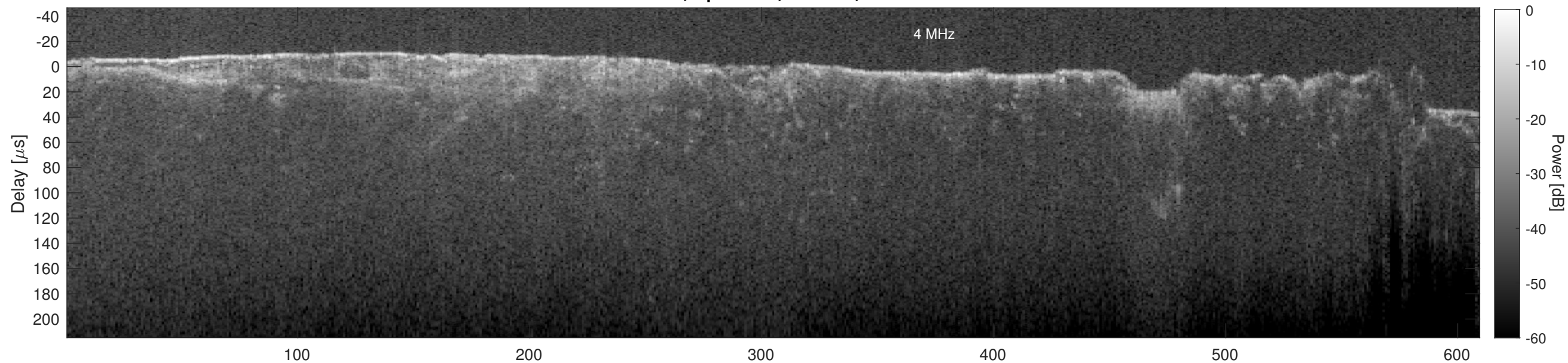
Orbit 6442, Cluttergram
