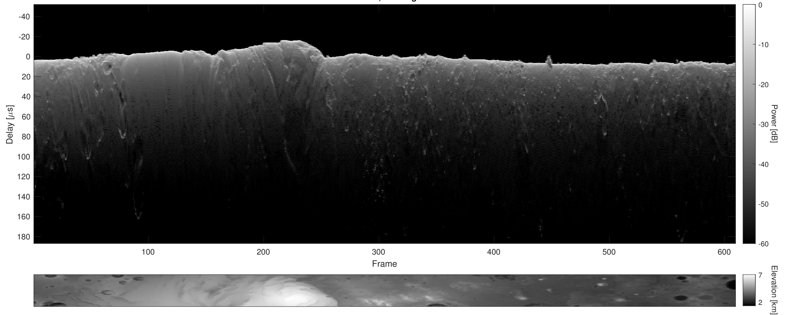
Orbit 6445, Cluttergram
