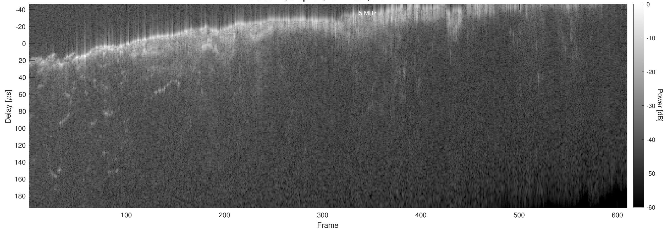
Orbit 6446, Chapman, No Window, Channel 2
