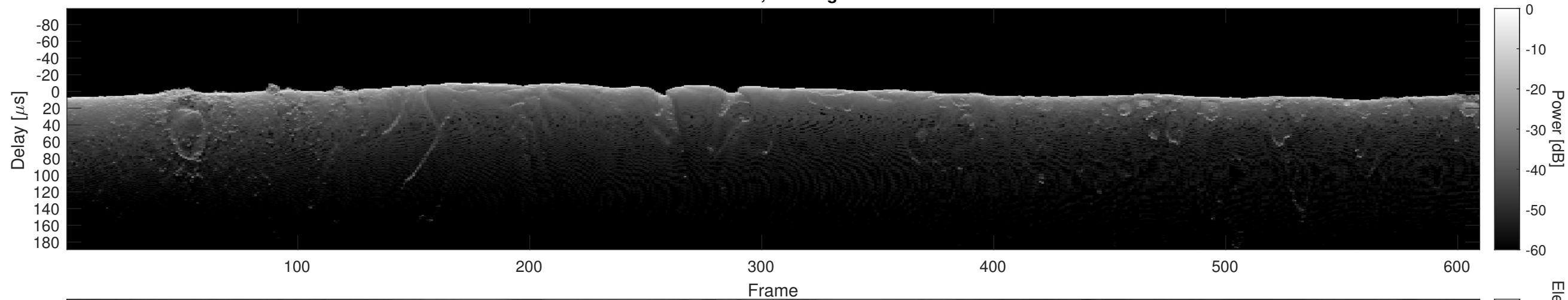
Orbit 6447, Cluttergram
