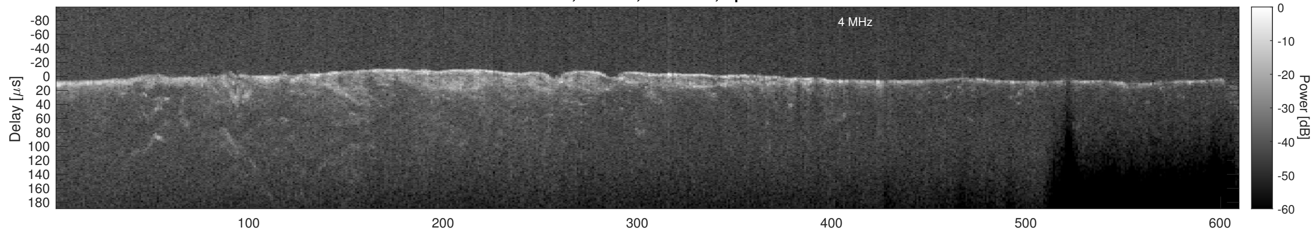
Orbit 6447, Cluttergram
