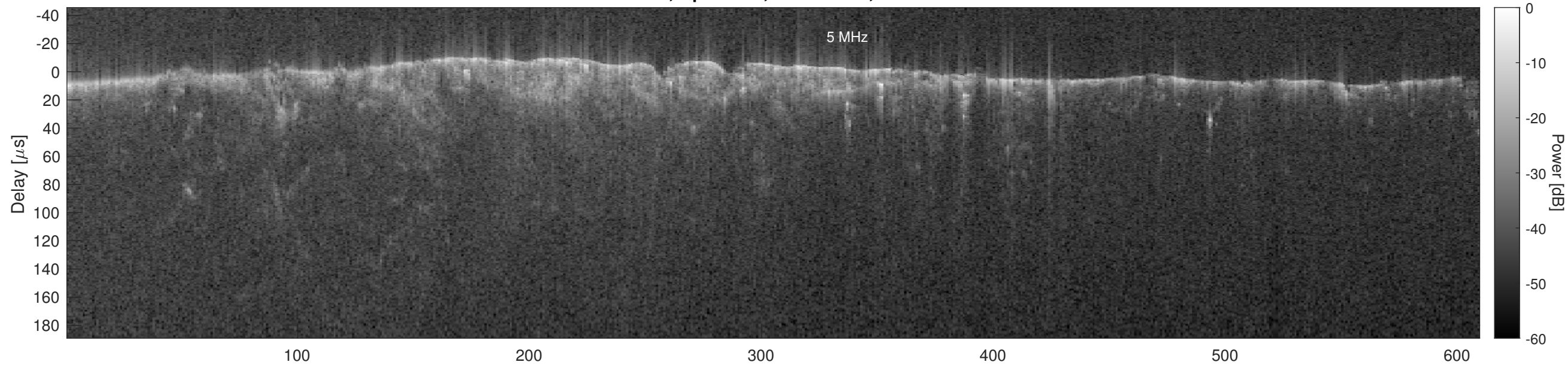
Orbit 6447, Optimized, No Window, Channel 2
