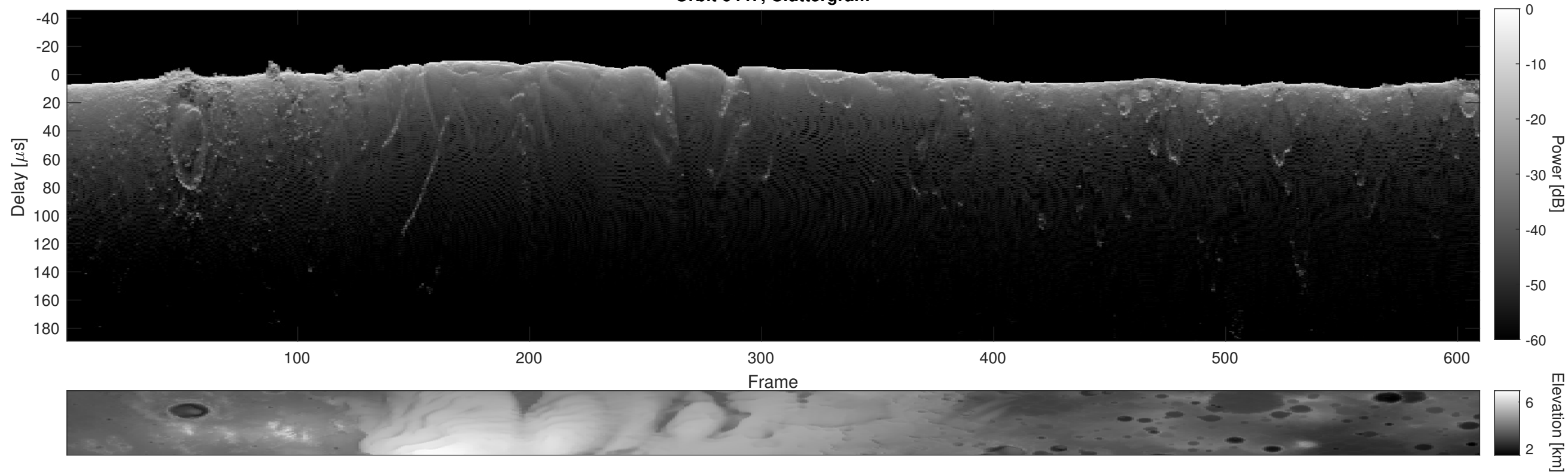
Orbit 6447, Cluttergram
