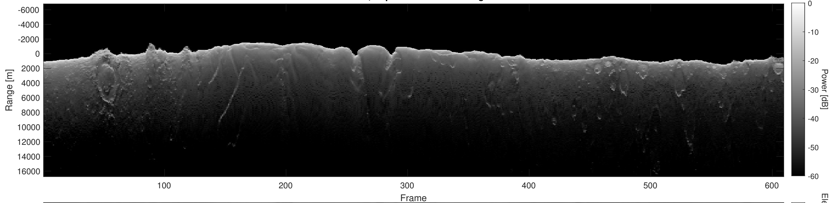
Orbit 6447, Depth-Corrected Cluttergram
