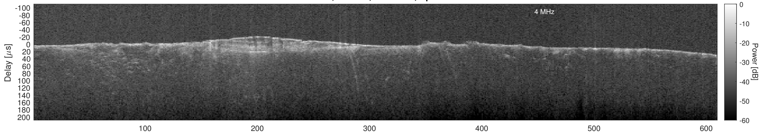
Orbit 6448, Cluttergram
