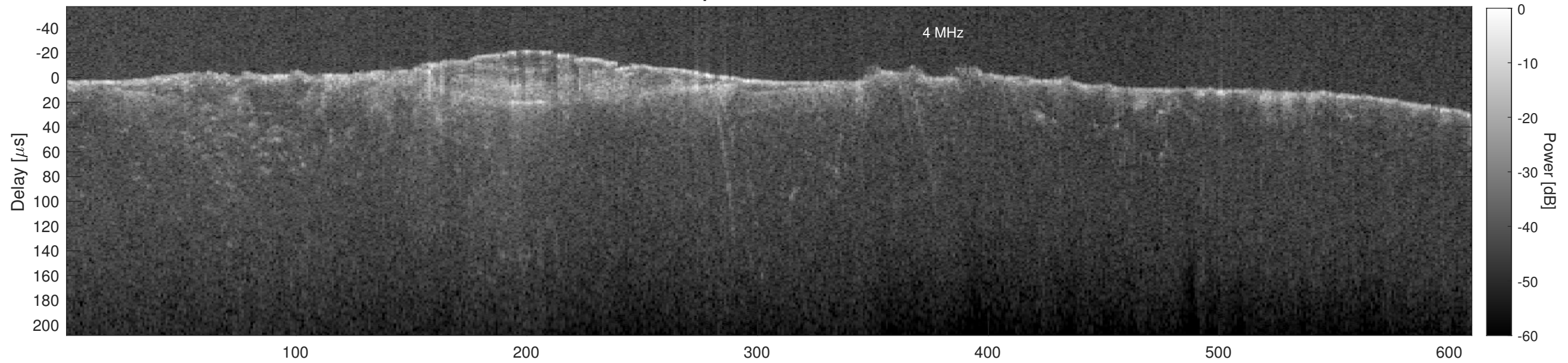
Orbit 6448, Cluttergram
