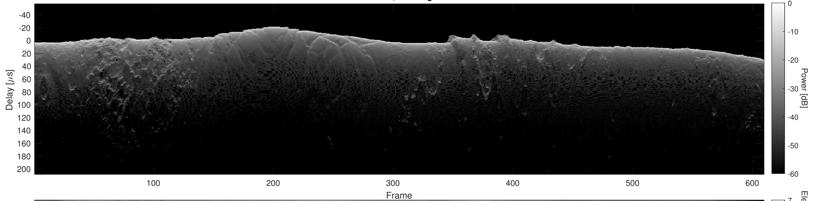
Orbit 6448, Cluttergram
